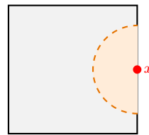
[0, 1]^2 \subseteq [0, 1]^2 ( open )
