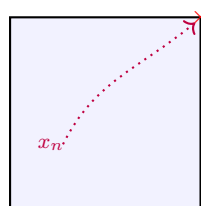
(a) [0, 1]^2 ( closed )
