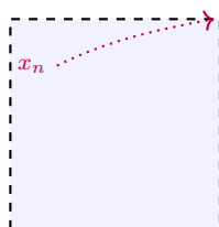
(b) (0, 1)^2 ( open )
