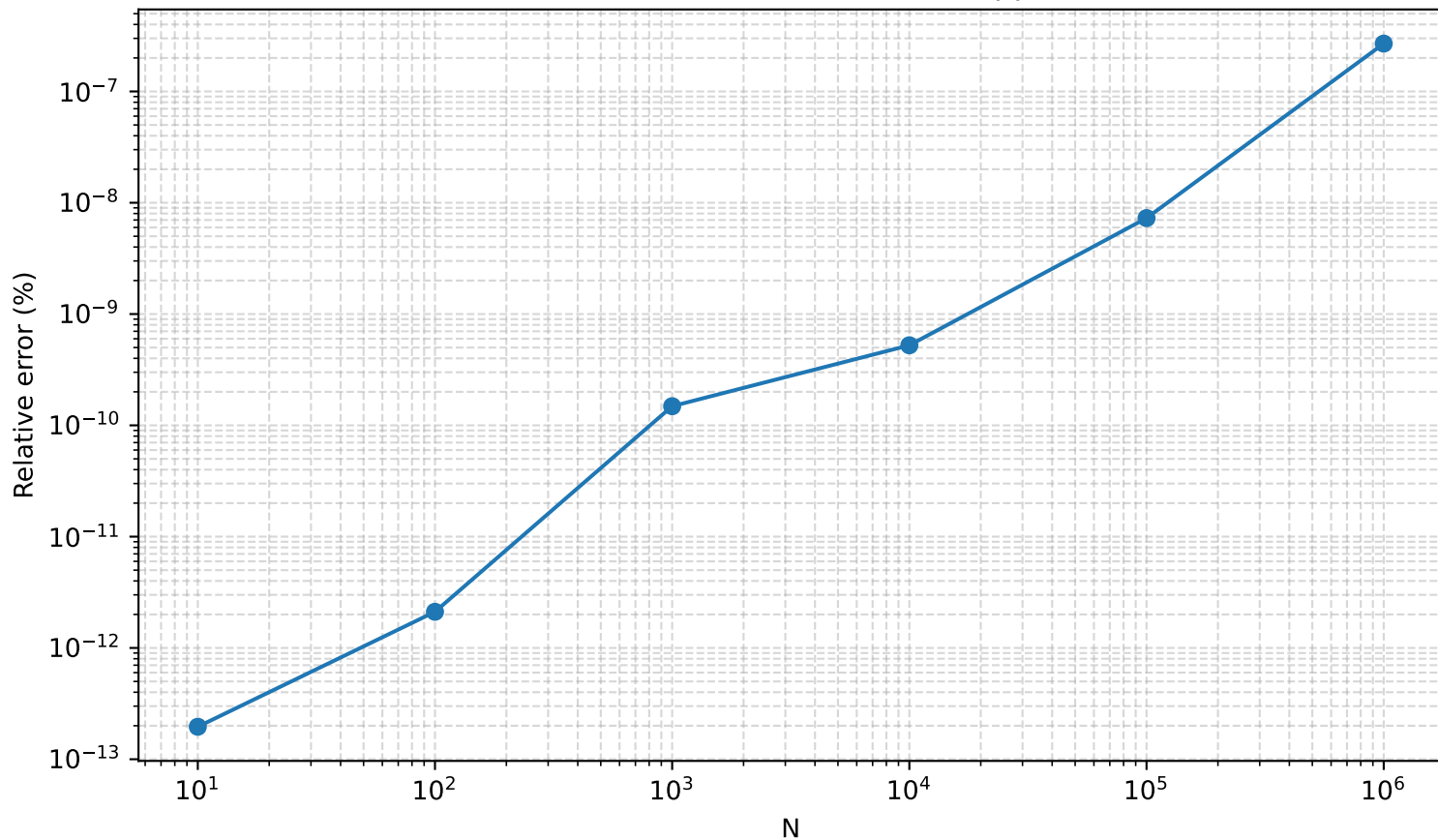
Relative Error of the Custom Factorial Approximation
