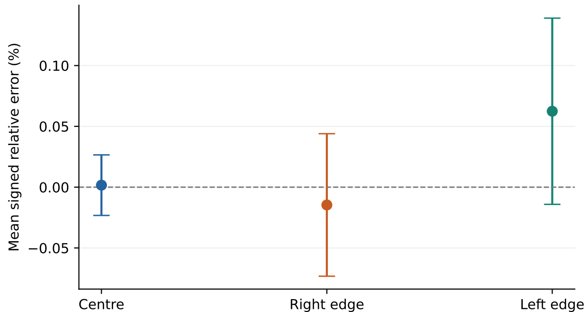
Residual offset at 4,096 SPP
