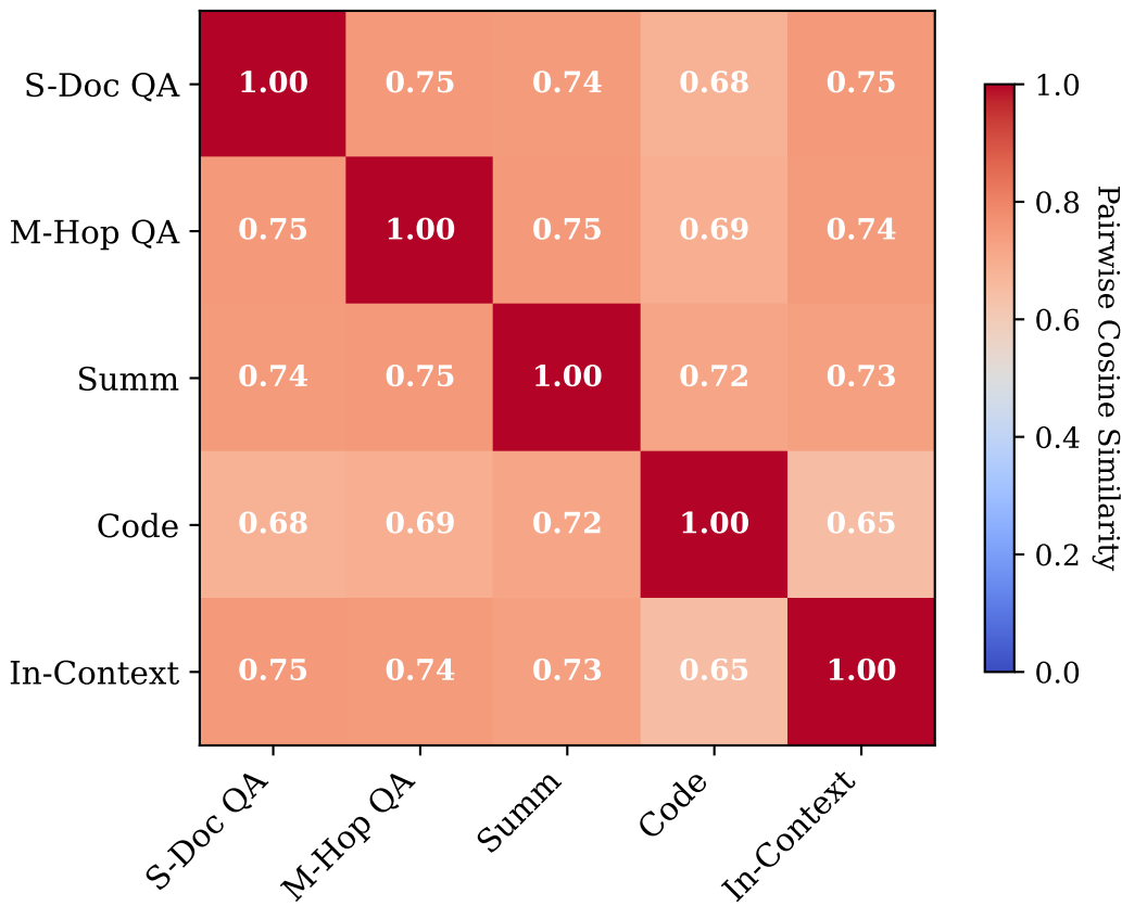
Pairwise Contrastive Similarity (Local Whitening per Pair) - Layer 0
