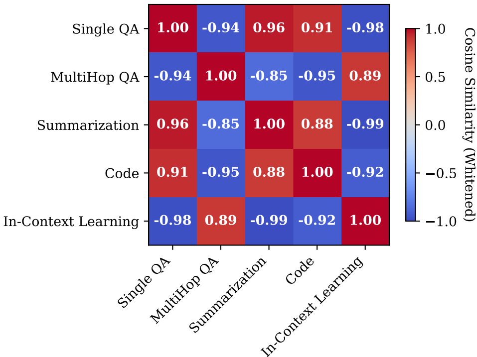
Task Similarity (Whitened Features) Layer 35
