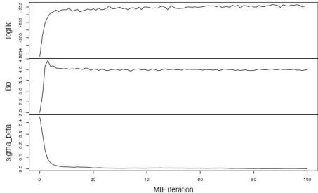
MIF2 convergence diagnostics
