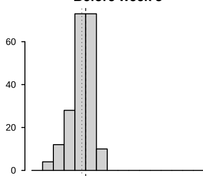
Before week 5
