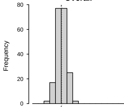
Overall
