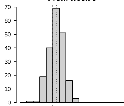
From week 5
