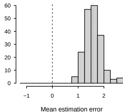
Constant-B
