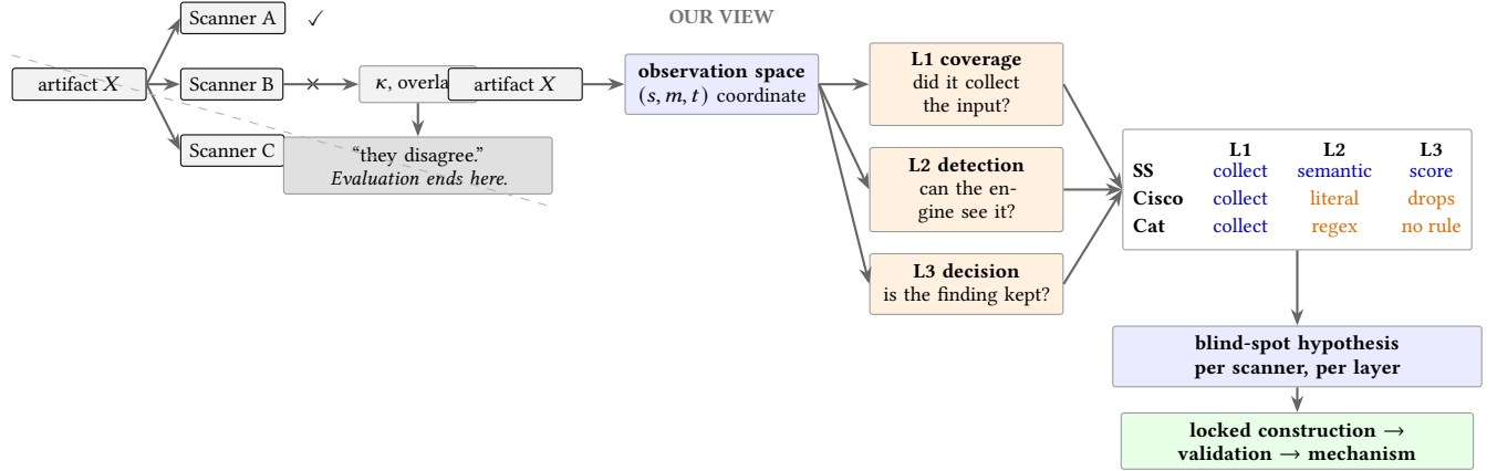
Figure 1: The same disagreement, read two ways. Current practice collapses three verdicts on artifact X into a scalar and stops. Our view localizes X in a shared observation space, decomposes each scanner’s failure into one architectural layer (coverage L1, detection L2, or decision L3), derives per-scanner blind-spot hypotheses, and validates them by construction locked before the fact.
