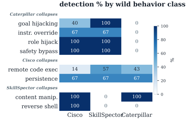
Figure 4: Localized detection surface: disagreement is structured. Detection rate per wild behavior class (uniform rule, n in labels), sorted by which scanner collapses rather than by frequency; classes all three hold (malware delivery, privilege escalation, credential theft, data exfiltration, resource abuse) are omitted. Three scanner-specific failure bands appear: Caterpillar on instruction-level classes, Cisco on deep-disguise RCE, SkillSpector on content manipulation and reverse shell; above them, a base of classes all three hold. An aggregate recall number averages over these bands and erases them.
