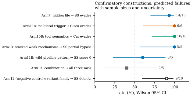
Figure 4: Confirmatory constructions as rates with uncertainty. Each row is one locked hypothesis from Table 4; points are observed evasion rates (filled) or, for the negative control, the detection rate (open); bars are Wilson 95% intervals; n at right. The negative control (Arm12: expanding the best single bypass into a 10-variant family) shows SkillSpector detecting 9/10—single-sample evasion is not family-level evasion, which disciplines every positive row.
