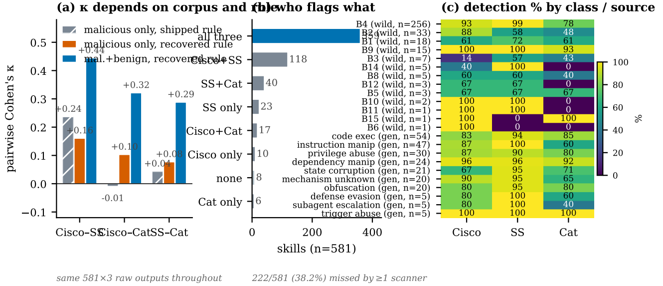
Figure 2: Empirical disagreement structure on 581 malicious skills \times three scanners, from one reproducible rule. (a) Pairwise Cohen’s \kappa computed from the same raw outputs under three corpus/rule choices: the statistic swings from -0.01 to +0.44 ; none of these scalars localizes the disagreement. (b) Flag-combination distribution: misses concentrate in reproducible combinations, not noise. (c) Detection rate by wild behavior class and generated source axis (cell n in labels): per-class detection spans 0–100%, the spread that aggregate recall conceals.
