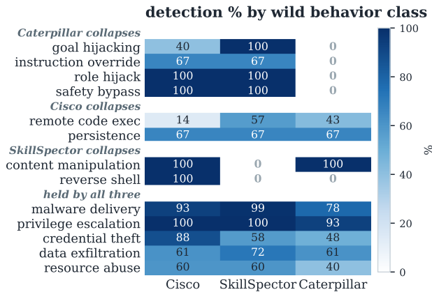
Figure 4: Localized detection surface: disagreement is structured. Detection rate per wild behavior class (all 13 classes, uniform rule, n in labels), sorted by which scanner collapses rather than by frequency. Three scanner-specific failure bands appear—Caterpillar on instruction-level classes, Cisco on deep-disguise RCE, SkillSpector on content manipulation and reverse shell—above a base of classes all three hold. An aggregate recall number averages over these bands and erases them.
