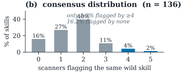
Figure 2: Disagreement is the norm in the wild. A market census (project week-0 data, no ground truth; its six scanners overlap with §5’s three only in SkillSpector): on 136 skills verified across platforms, all six public scanners’ pairwise Cohen’s \kappa \leq 0.244 with most near zero (a), and only 5.9% of skills are flagged by four or more scanners (b). On the full 1,082-skill census, 260 of 445 flagged skills are flagged by exactly one scanner. Disagreement at this scale is not noise to average away; it is the ecosystem’s default output.
