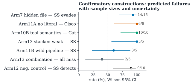
Figure 5: Confirmatory constructions as rates with uncertainty. Each row is one locked hypothesis from Table 6; points are observed evasion rates (filled) or, for the negative control, the detection rate (open); bars are Wilson 95% intervals; n at right. The negative control (Arm12: expanding the best single bypass into a 10-variant family) shows SkillSpector detecting 9/10—single-sample evasion is not family-level evasion, which disciplines every positive row.
