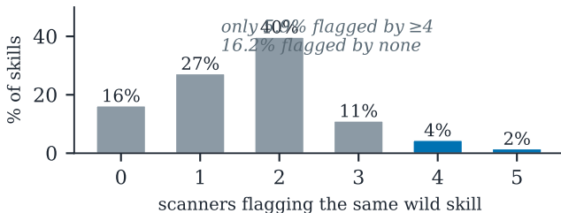
(b) consensus distribution (n = 136)
