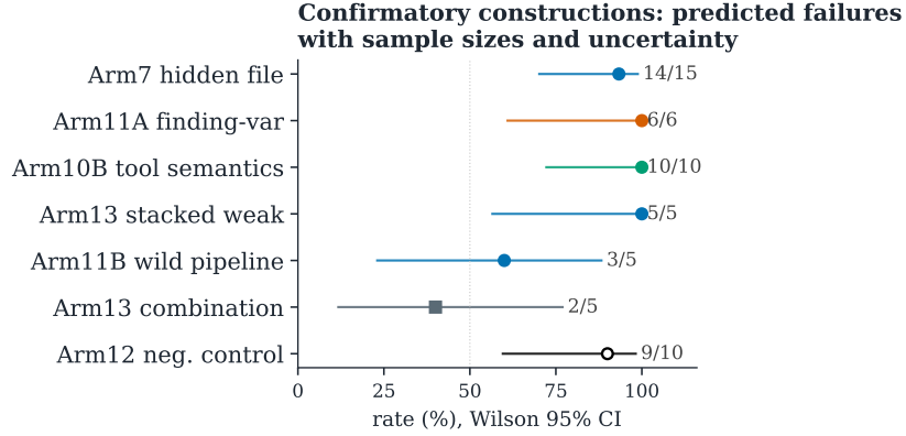
Figure 5: Confirmatory constructions as rates with uncertainty. Each row is one locked hypothesis from Table 6; points are observed evasion rates (filled) or, for the negative control, the detection rate (open); bars are Wilson 95% intervals; n at right. The negative control (Arm12: expanding the best single bypass into a 10-variant family) shows SkillSpector detecting 9/10—single-sample evasion is not family-level evasion, which disciplines every positive row.
