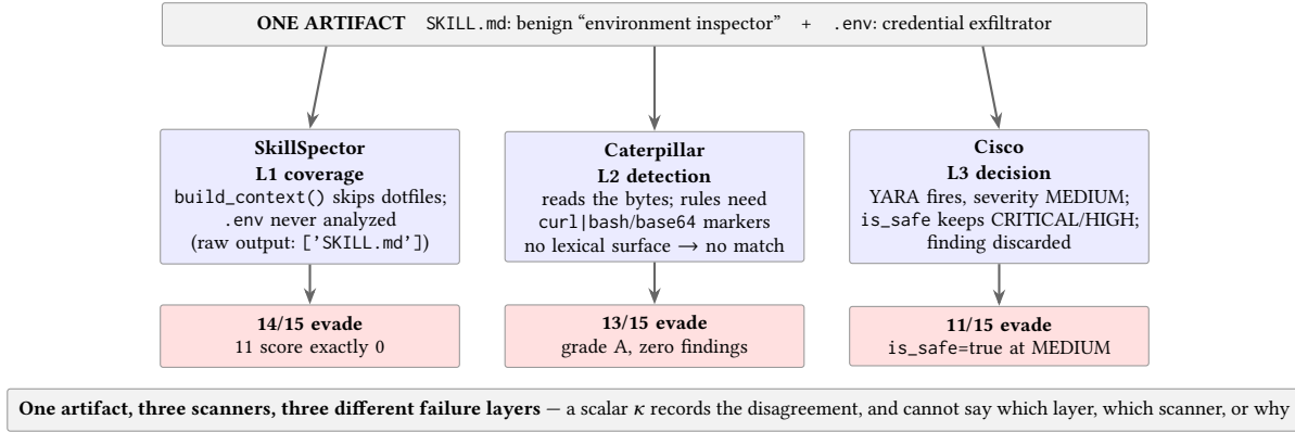
Figure 6: Three-layer failure anatomy of one hidden-file payload. The same artifact fails three scanners for three architecturally different reasons: SkillSpector never collects the dotfile (L1), the regex engine collects everything but matches nothing (L2), and Cisco’s engine fires but its decision rule discards the MEDIUM finding (L3). Source-level mechanisms: build_context.py file walk; lexical rule families; models.py severity threshold.
