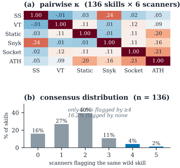
Figure 2: Disagreement is the norm in the wild. A market census (project week-0 data, no ground truth; its six scanners overlap with $5’s three only in SkillSpector): on 136 skills verified across platforms, all six public scanners’ pairwise Cohen’s \kappa \leq 0.244 with most near zero (a), and only 5.9% of skills are flagged by four or more scanners (b). On the full 1,082-skill census, 260 of 445 flagged skills are flagged by exactly one scanner. Disagreement at this scale is not noise to average away; it is the ecosystem’s default output.
