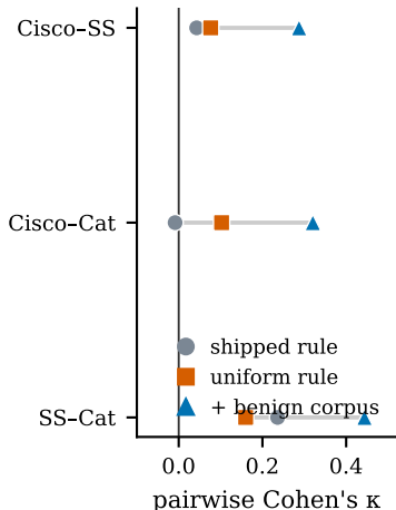
(a) same outputs, three \kappa values
