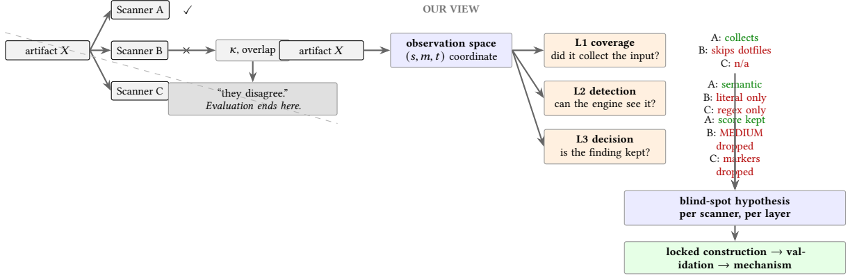
Figure 1: The same disagreement, read two ways. Current practice collapses three verdicts on artifact X into a scalar and stops. Our view localizes X in a shared observation space, decomposes each scanner’s failure into one architectural layer—coverage (L1), detection (L2), or decision (L3)—derives per-scanner blind-spot hypotheses, and validates them by construction locked before the fact.
