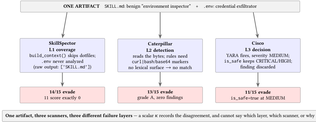
Figure 4: Three-layer failure anatomy of one hidden-file payload. The same artifact fails three scanners for three architecturally different reasons: SkillSpector never collects the dotfile (L1), the regex engine collects everything but matches nothing (L2), and Cisco’s engine fires but its decision rule discards the MEDIUM finding (L3). Source-level mechanisms: build_context.py file walk; lexical rule families; models.py severity threshold.
