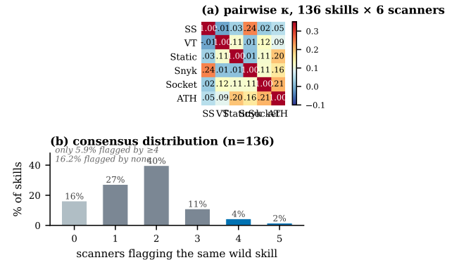
Figure 2: Disagreement is the norm in the wild. A market census (project week-0 data, no ground truth; scanner set distinct from §5): on 136 skills verified across platforms, all six public scanners’ pairwise Cohen’s \kappa \leq 0.244 with most near zero (a), and only 5.9% of skills are flagged by four or more scanners (b). On the full 1,082-skill census, 260 of 445 flagged skills are flagged by exactly one scanner. Disagreement at this scale is not noise to average away; it is the ecosystem’s default output.
