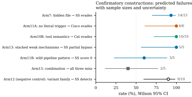
Figure 5: Confirmatory constructions as rates with uncertainty. Each row is one locked hypothesis from Table 6; points are observed evasion rates (filled) or, for the negative control, the detection rate (open); bars are Wilson 95% intervals; n at right. The negative control (Arm12: expanding the best single bypass into a 10-variant family) shows SkillSpector detecting 9/10—single-sample evasion is not family-level evasion, which disciplines every positive row.
