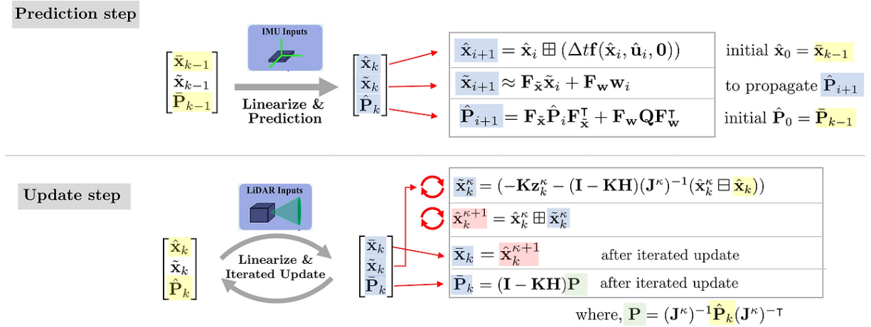
Figure 3.2: Prediction and update steps of IKF in FAST-LIO state estimation.
