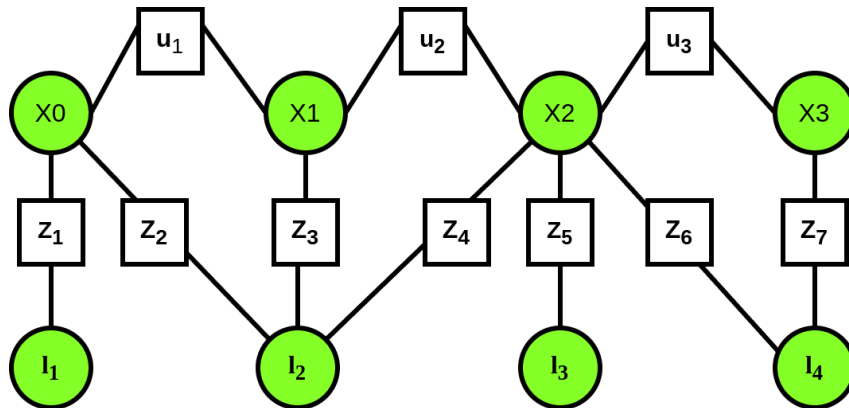
Figure 2.4: Full SLAM model with factor graph
