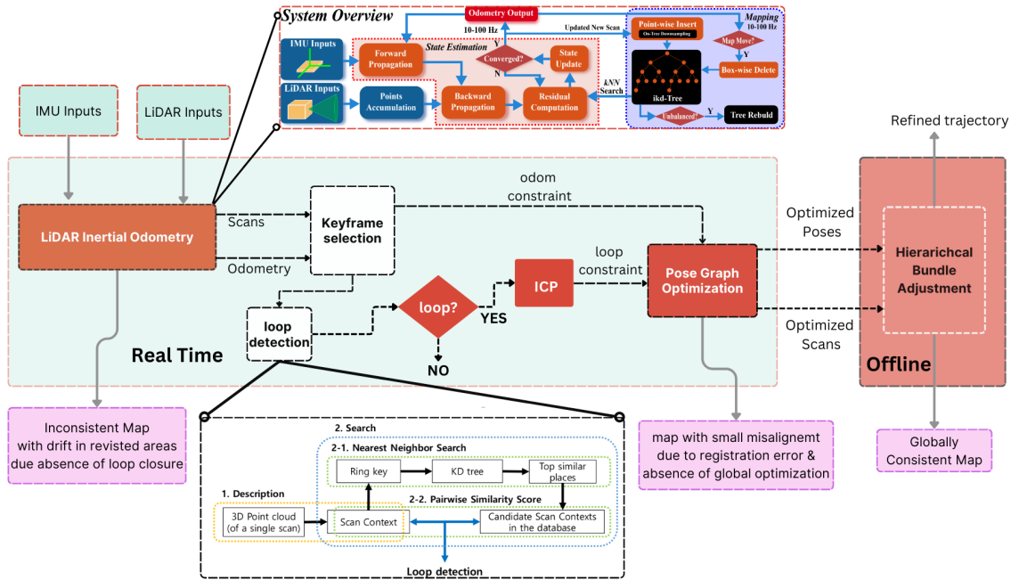
Figure 3.1: Block diagram of the overall system pipeline.
