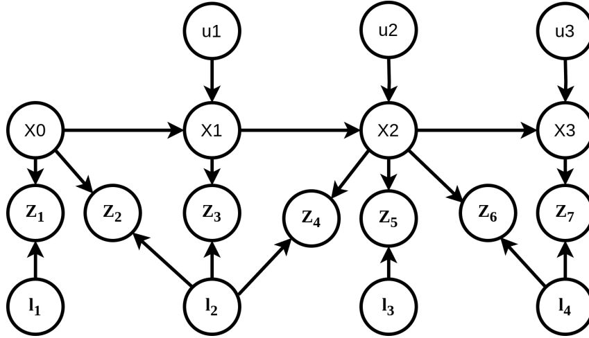
Figure 2.3: Probabilistic Bayesian net SLAM model
