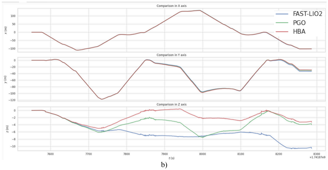
Figure 4.2: Comparison of trajectories for Saxion_01 dataset. a) Top view trajectories. b) Axis-wise comparison
