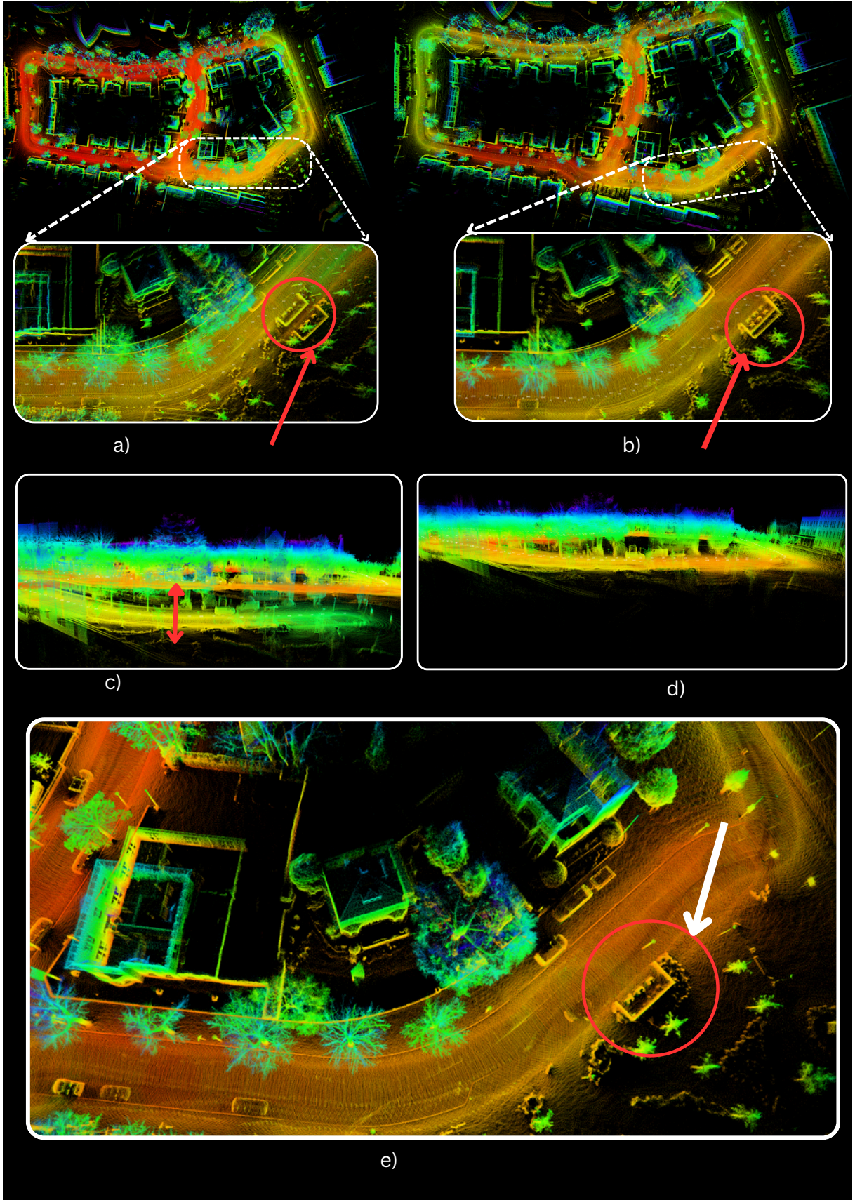
Figure 4.3: Map generated by each stage of the mapping pipeline. a) FAST-LIO2 top view. b) PGO top view. c) FAST-LIO side view. d) PGO side view. e) HBA
