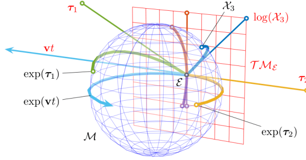
Figure 2.1: Relationship between Lie Groups and Lie algebras
