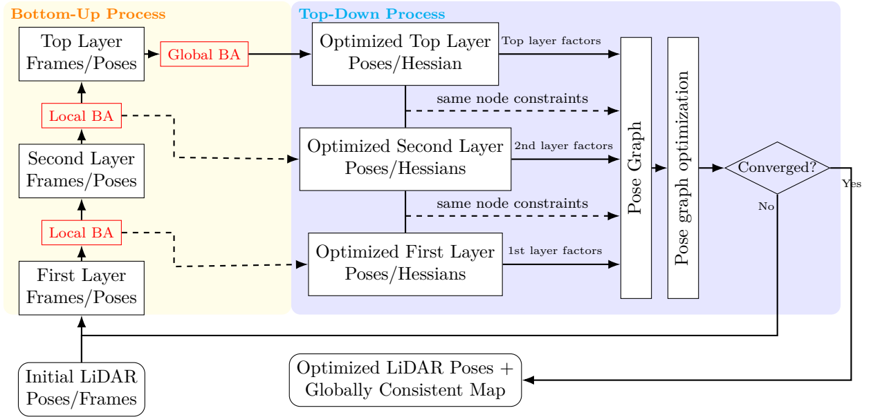
Figure 3.8: HBA optimization: Bottom-Up and Top-Down Process[18]
