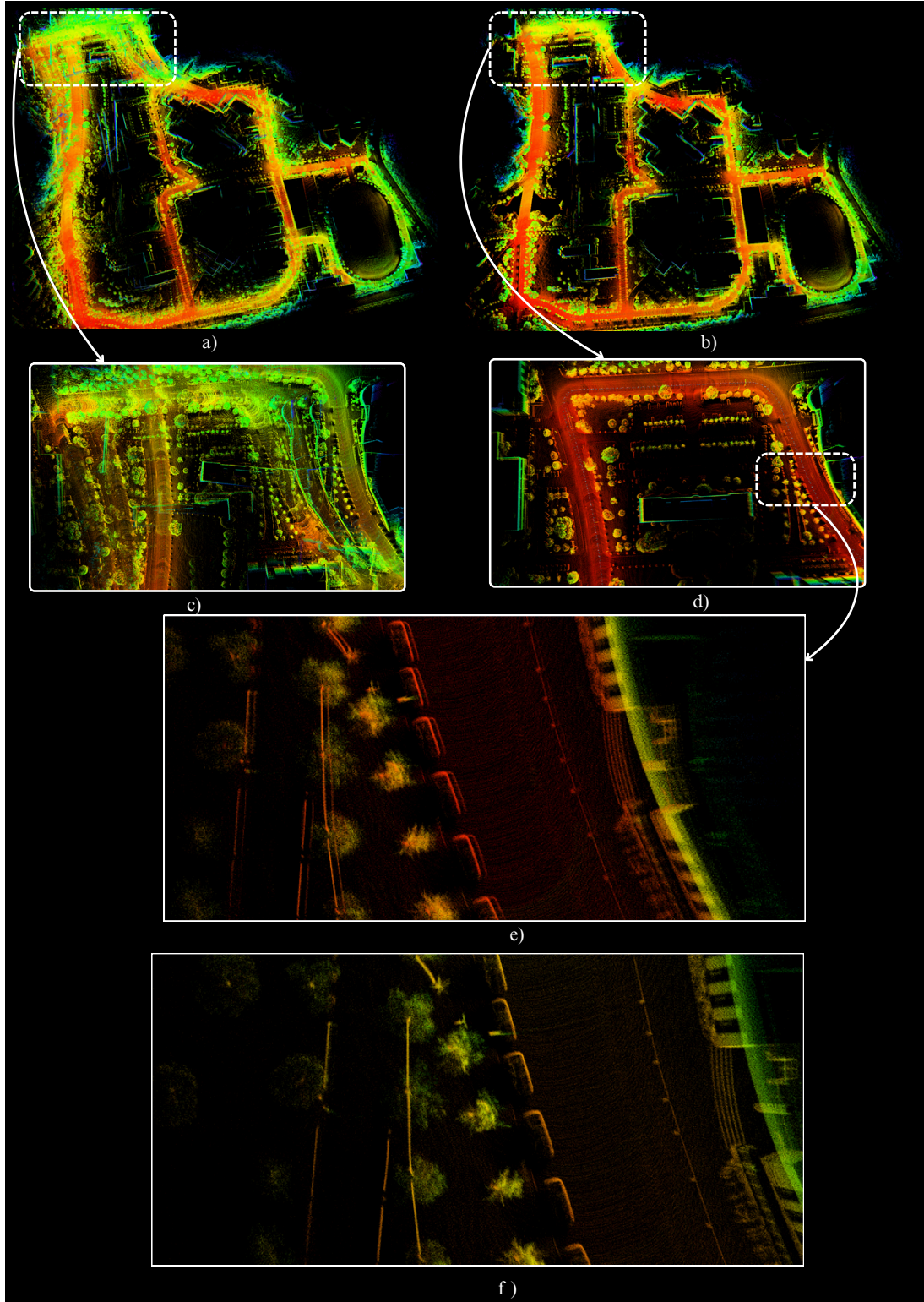
Figure 2: Map generated by each stage of the mapping pipeline for MulRan KAIST dataset sequence 03. a) Map generated by FAST-LIO2, b) Map after optimizing with PGO, c) and d) show segments from a) and b) zoomed in respectively. e) shows the existence of divergence in the map even after PGO. f) shows the map in e) after correction with HBA.
