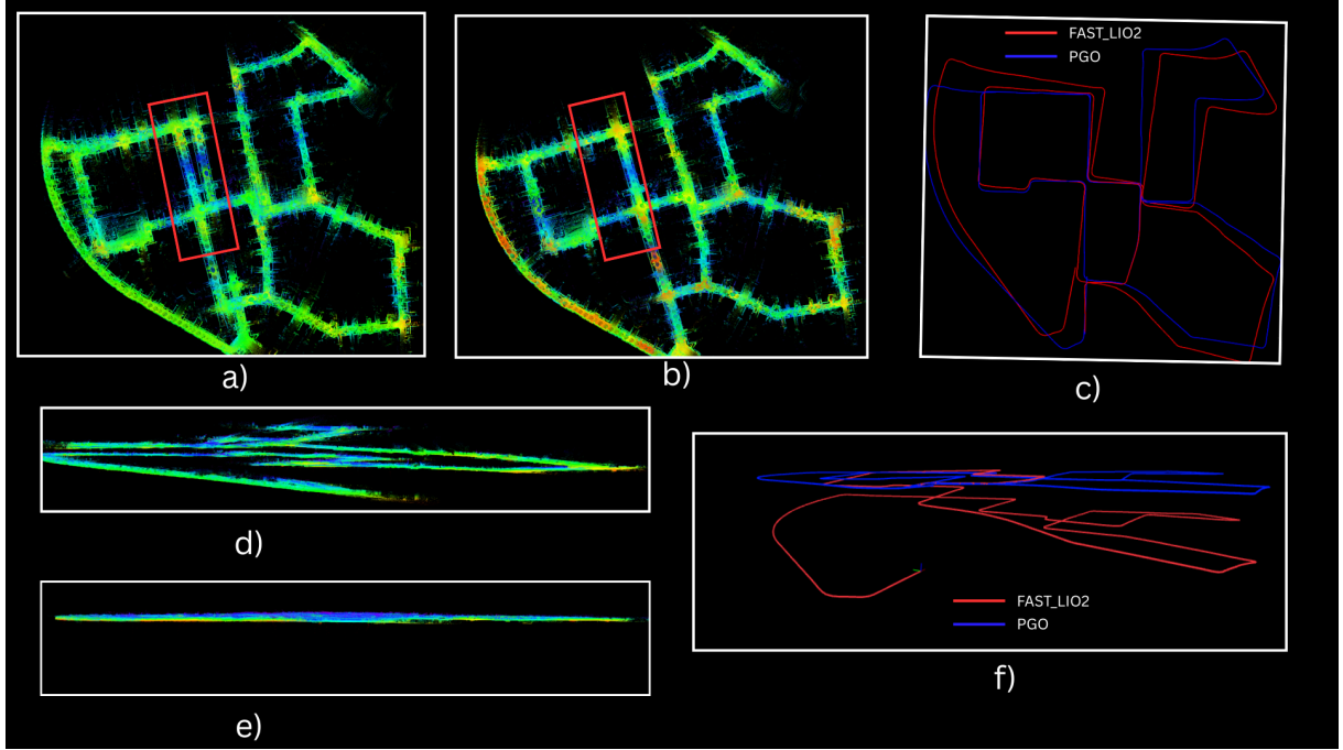
Figure 3: Map visualization for KITTI00 sequence. a) BEV of map generated by FAST-LIO2. b) BEV of map after PGO optimization. c) BEV of FAST-LIO2 and PGO trajectories. d) Side view of FAST-LIO2 map. e) Side view the optimized map. f) Side view of FAST-LIO2 and PGO trajectories
