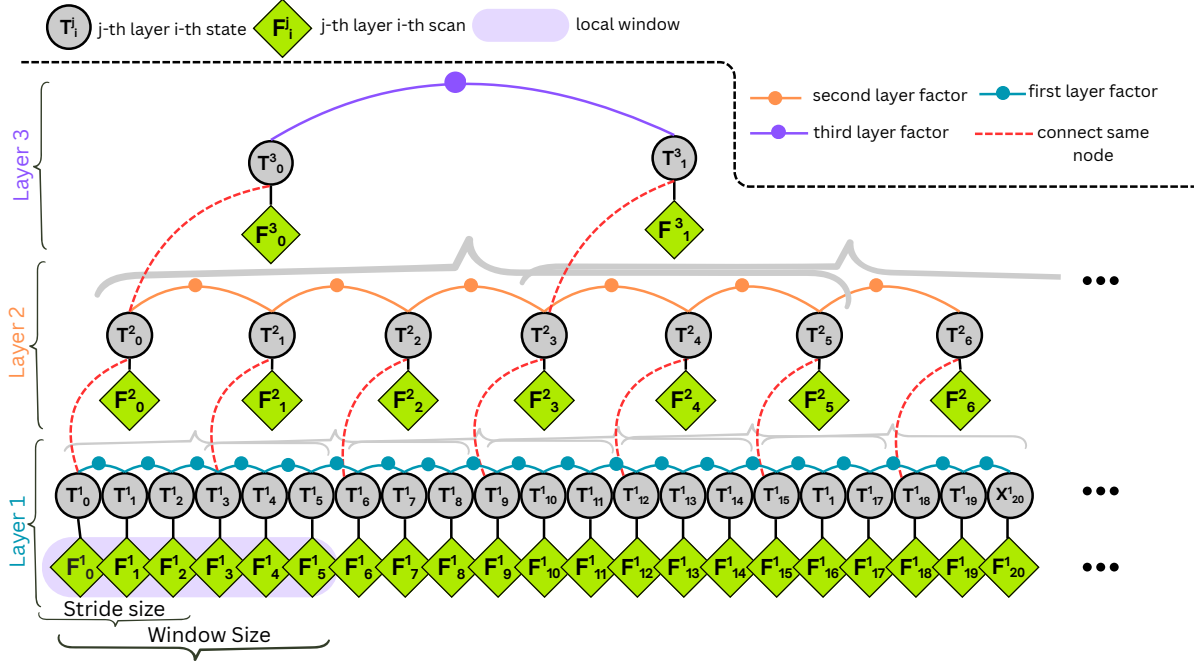
Figure 3.7: Pyramid structure of the HBA with layer number l=3 , stride size s=3 and window size w=6 .
