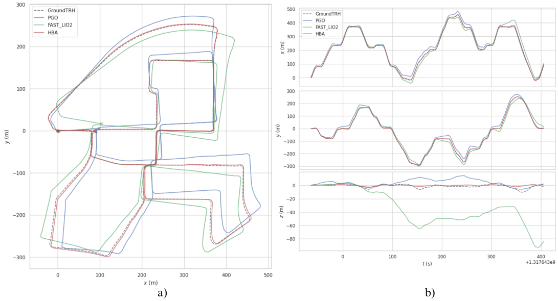
Figure 4: Visualization of trajectories for KITTI00. a) BEV trajectories . b) Axis-wise comparison of the trajectories.
