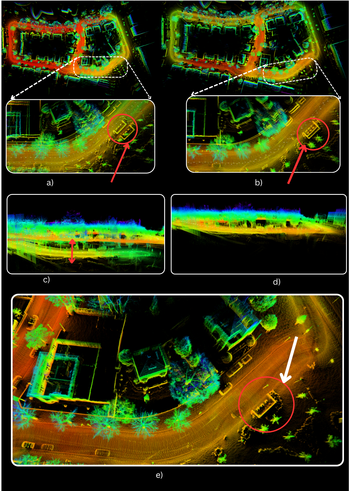
Figure 4.3: Map generated by each stage of the mapping pipeline for saxion01. a) FAST-LIO2 top view. b) PGO top view. c) FAST-LIO side view. d) PGO side view. e) HBA
