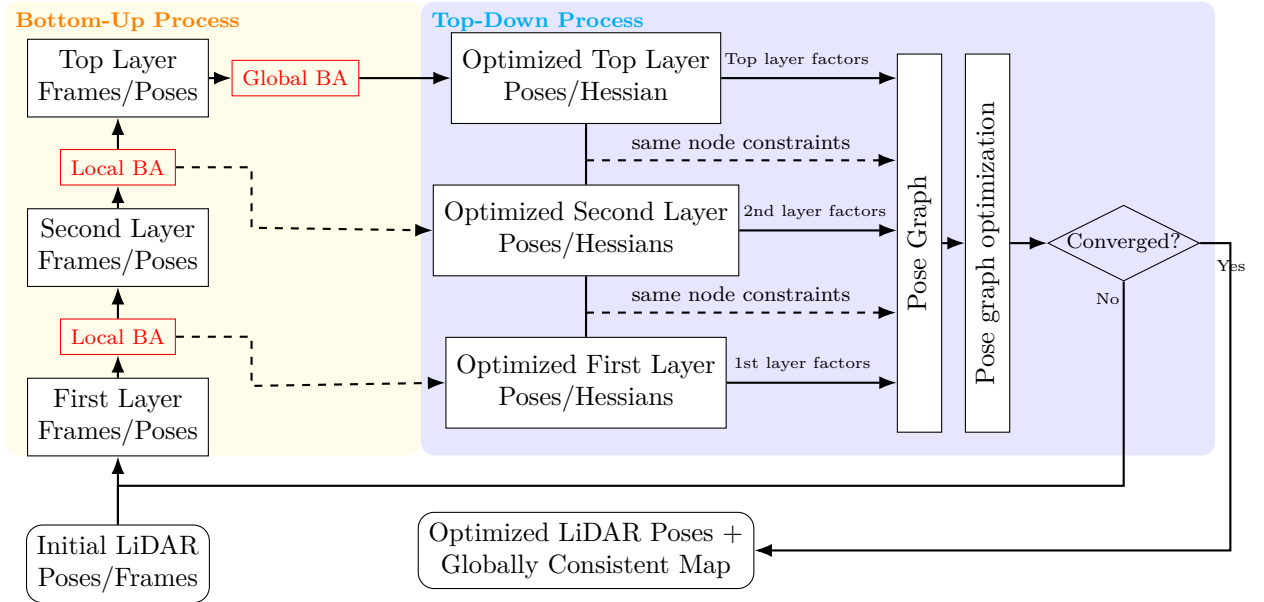
Figure 3.8: HBA optimization: Bottom-Up and Top-Down Process
