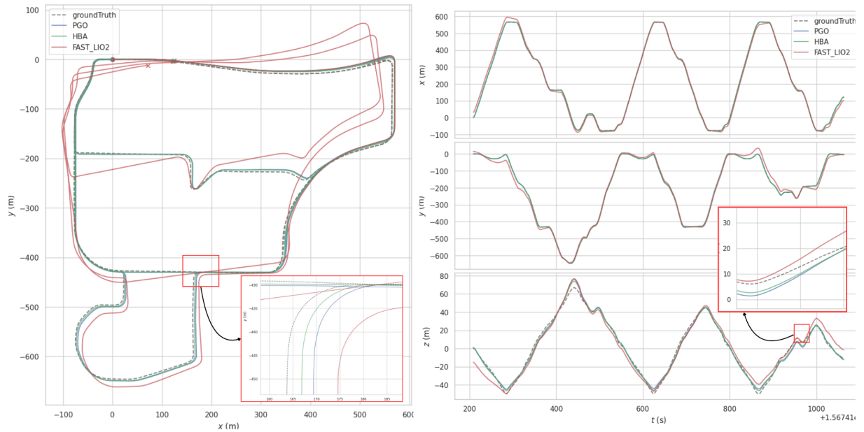
Figure 1: Trajectories for MulRan KAIST03 sequence. a) Comparison of FAST-LIO2, PGO, and HBA trajectories with ground truth trajectory. b) Axis-wise comparison
