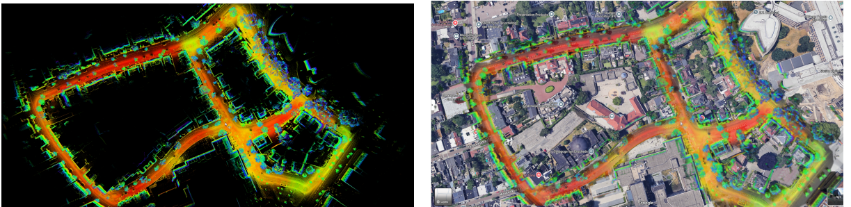
Figure 4.4: Mapping result for saxion03
