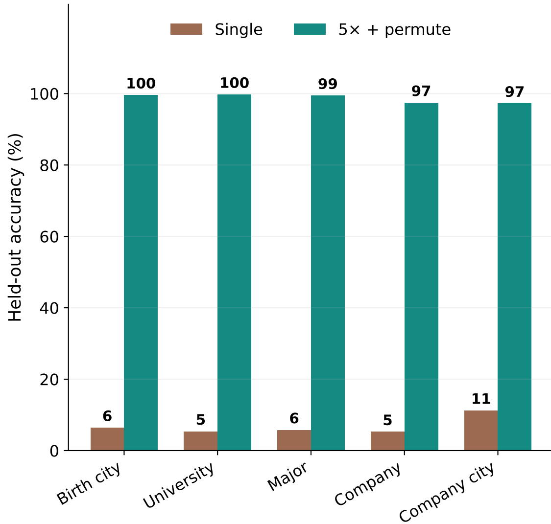
B P0 probe · first token
