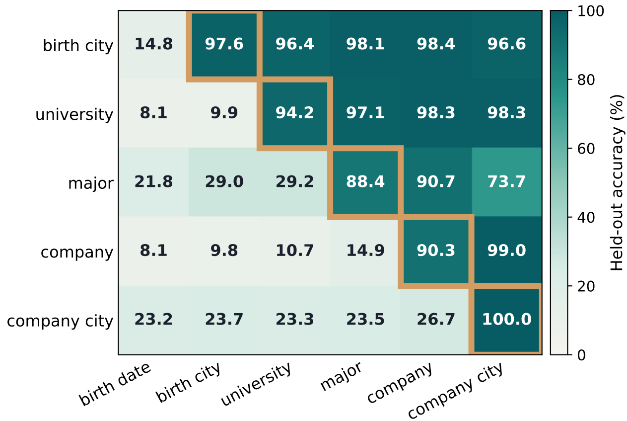
Fresh whole probe + P-first output fixed positions outlined
