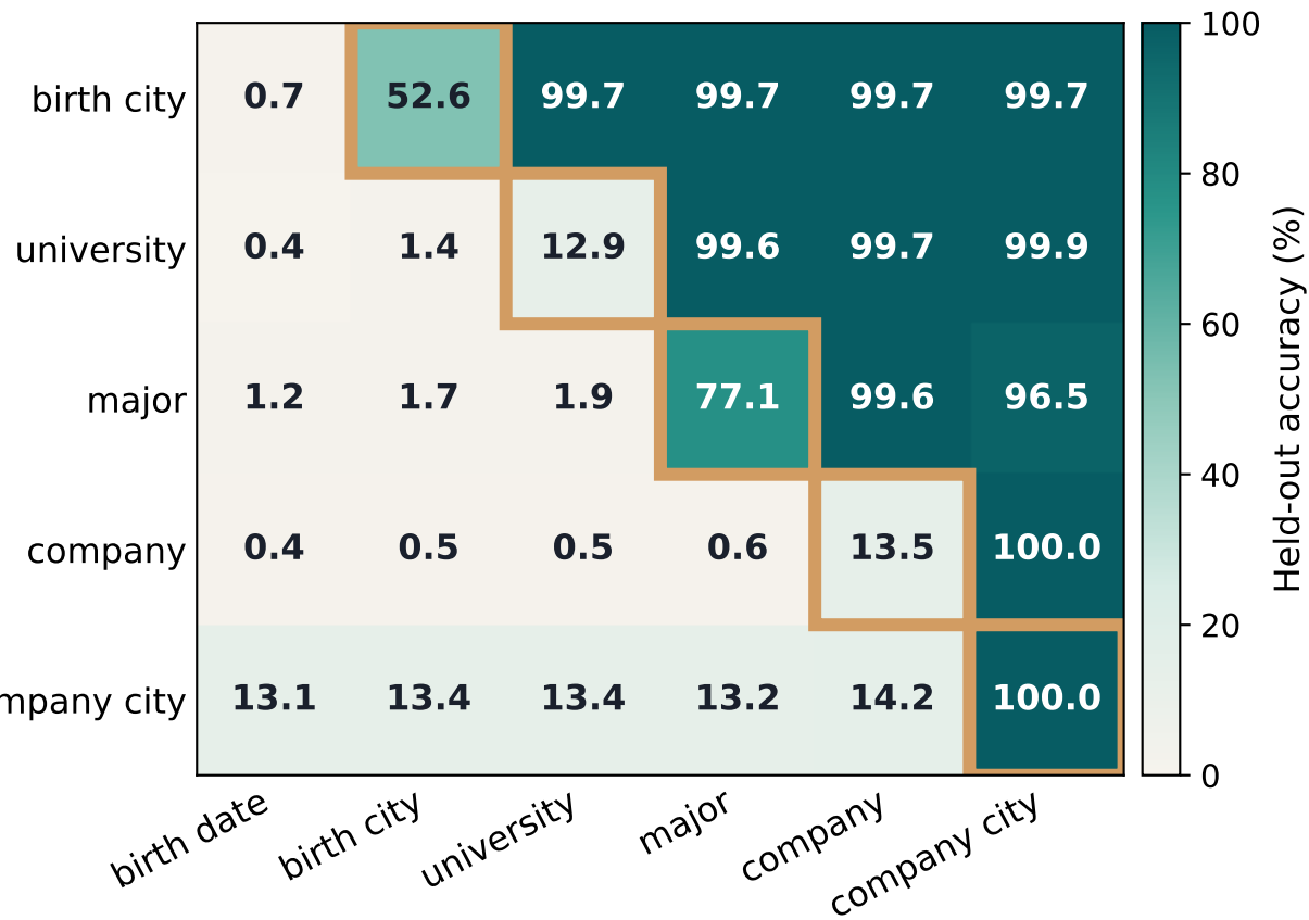
Formal no-t1 baseline fixed positions outlined
