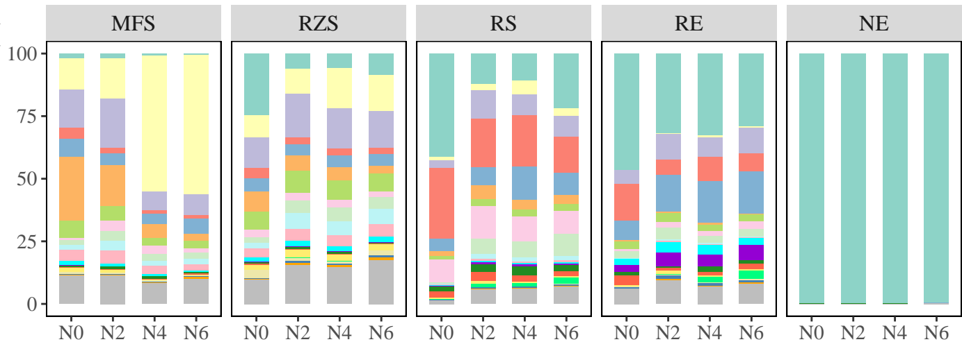
Rhizobia Relative Abundance(%)
