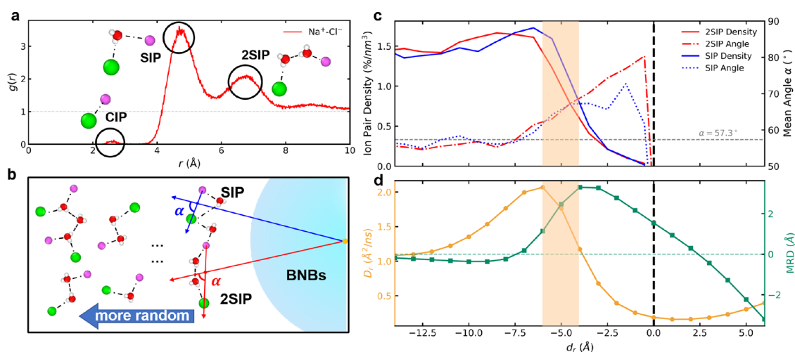
Figure 7. Analysis of ion pairs and the radial diffusion dynamics of nitrogen molecules in the saline system. (a) Radial distribution function, g(r) , of \text{Na}^+-\text{Cl}^- pairs, where distinct peaks identify three ion-pairing modes: contact ion pair (CIP), solvent-separated ion pair (SIP), and double solvent-separated ion pair (2SIP). (b) Schematic illustration of SIP and 2SIP configurations near the gas–liquid interface, defining the orientation angle \alpha relative to the radial vector. In panels (a) and (b), purple and green spheres represent \text{Na}^+ and \text{Cl}^- ions, respectively. (c) Radial profiles showing the normalized number density and mean orientation angle of SIP and 2SIP as a function of distance from the interface. The gray horizontal dashed line denotes the spatial average orientation angle \alpha of 57.3^\circ that exhibits randomly oriented ion pairs in the bulk water region. (d) Spatially resolved dynamics of nitrogen molecules, characterized by the radial diffusion coefficient ( D_r ) and mean radial displacement (MRD) of nitrogen molecules near the interface. The vertical dashed lines in (c) and (d) denote the position of the GDS. Panels (c) and (d) were calculated from three independent ripening trajectories in the saline system.
