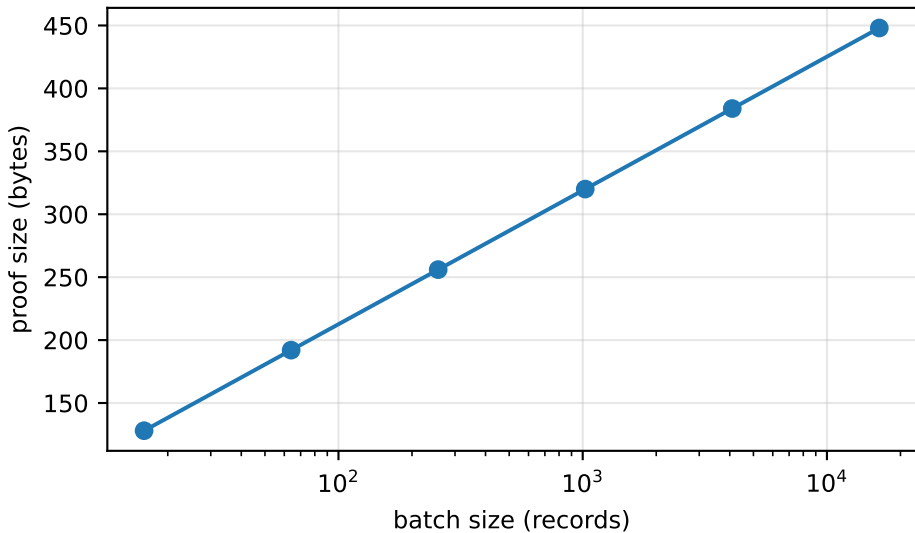
Inclusion proof size is logarithmic in batch size
