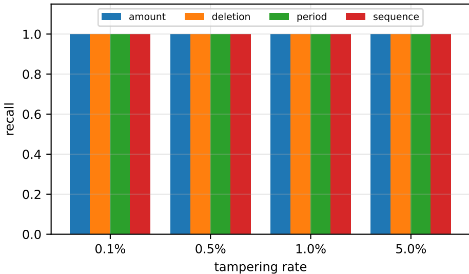
Detection rate by attack class
