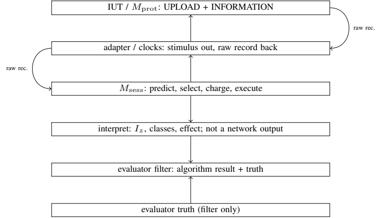
Fig. 1. Context derived from FIG-CL-TAV-01/07. Stimulus and raw records share ports. Truth enters only the evaluator filter, never select, predict, history or execute.
