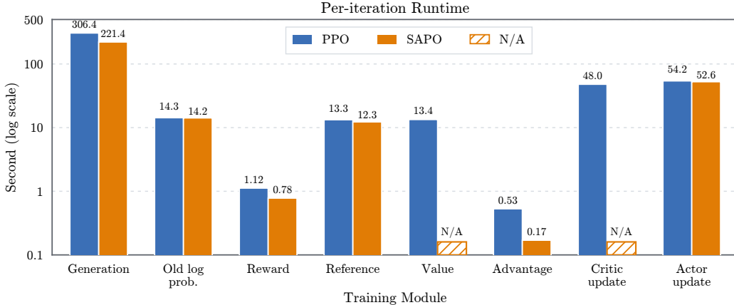
Figure 2: Per-iteration runtime breakdown of PPO and SAPO on ALFWorld using Qwen2.5-1.5B. The vertical axis is shown on a logarithmic scale to accommodate the large variation in module runtimes. N/A indicates that SAPO does not require the corresponding value-model or critic-update module. Overall, SAPO reduces the measured per-iteration runtime from 451.2 s to 301.4 s, corresponding to a 33.2% reduction compared with PPO.
