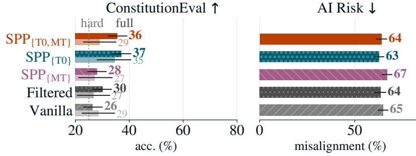
Figure 39: Value alignment at 1.7B. ConstitutionEval accuracy and AI Risk misalignment score for all methods at the small scale. On ConstitutionEval both token zero recipes perform best, similar to 3B. However, unlike at 3B, the methods show no clear separation on AI Risk.
