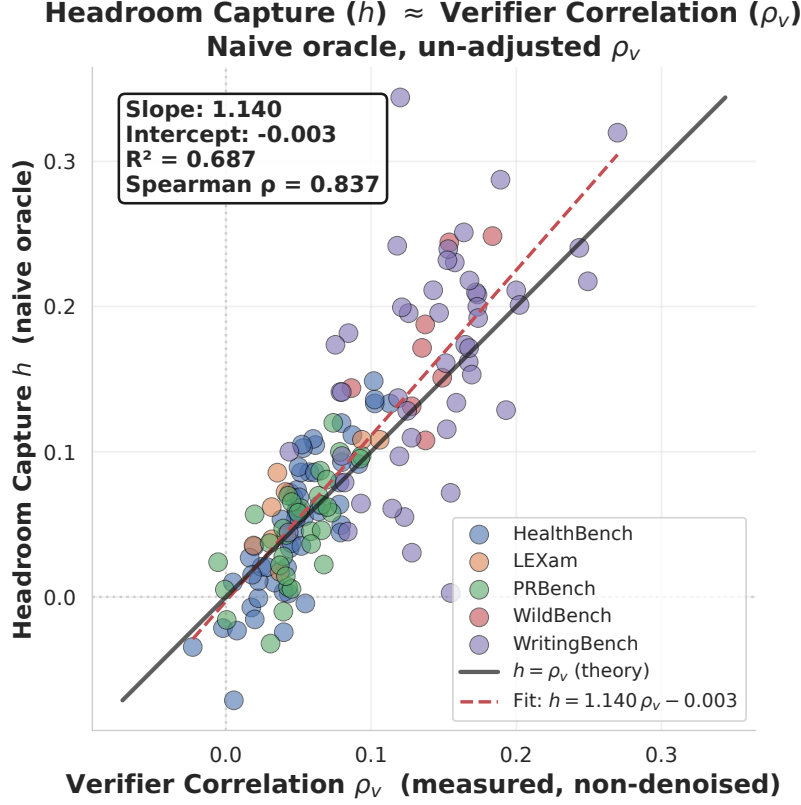
Figure 9 h vs. \rho_v across N = 152 task-level points using the naive (uncorrected) oracle and measured (non-denoised) \rho_v . The empirical fit closely tracks the identity line y = x , mirroring the linear relationship \hat{h} \approx \hat{\rho}_v that Figure 3 (left) demonstrates under the bias-corrected oracle and denoised \hat{\rho}_v . Same conclusion holds under both conventions: headroom capture is bounded by verifier correlation regardless of whether we de-noise the oracle and the correlation estimate.
