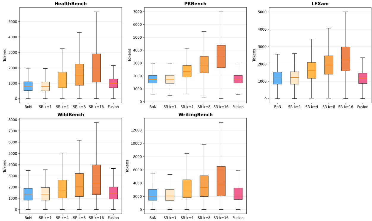
Figure 12 Token length distributions per method and benchmark for Qwen3.5-35B-A3B. BoN (blue) and Fusion (pink) show stable length distributions across compute levels. Sequential Refinement (orange gradient, SR k=1 through k=16 ) shows monotonically increasing median length on every benchmark, with the steepest growth on WritingBench and PRBench.
