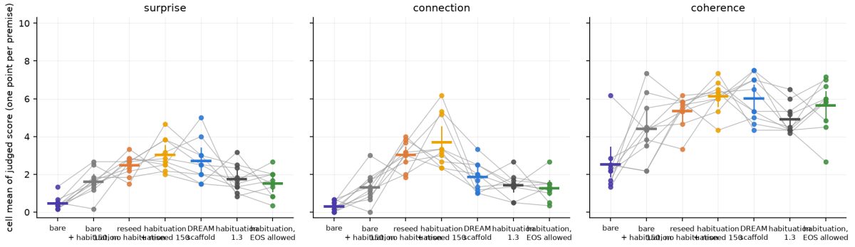
Figure 2: Habituation and interruption: bare, bare + habituation, interruption without habituation, habituation + interruption 150, the full scaffold, and the two habituation baselines (stronger penalty; EOS allowed). One point per premise, grey lines join the same premise across arms, bars are cell means with 95% bootstrap CIs over cells (Qwen3-30B-A3B, generated-only windows).
