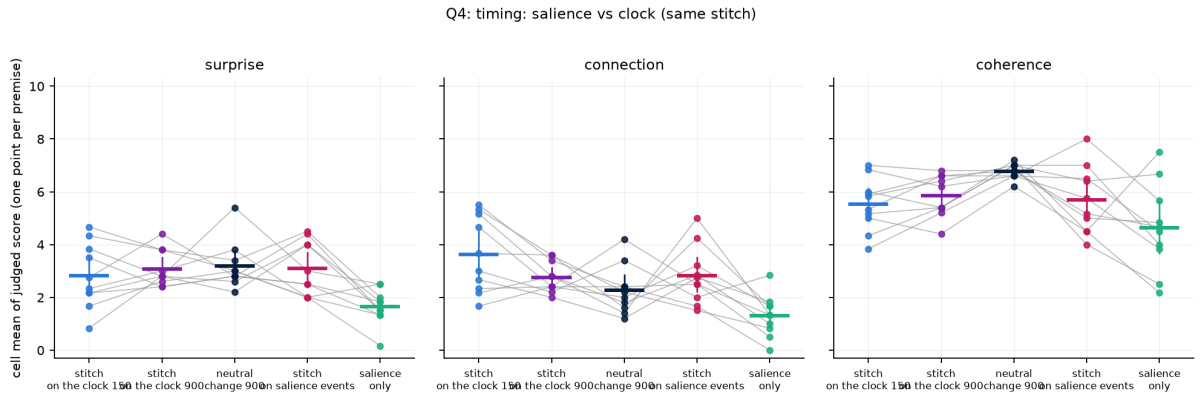
Figure 5: When to interrupt: the re-encounter stitch on the clock (150 and 900), the neutral change every 900, the stitch on salience events, and salience only (nothing injected). Post-interruption windows; one point per premise.
