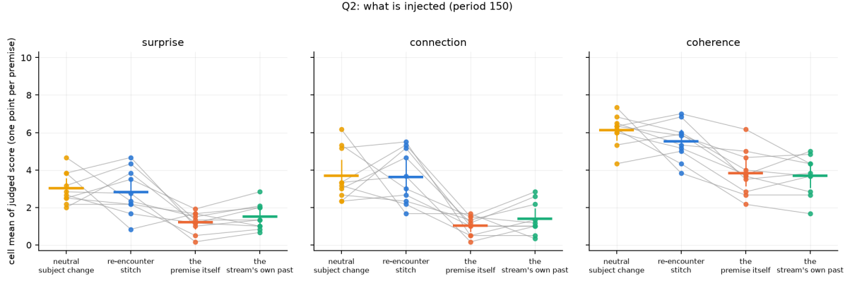
Figure 4: Content of the interruption at period 150: neutral change, re-encounter stitch, the premise itself, the stream’s own past. Injecting a return is as bad as not interrupting.
