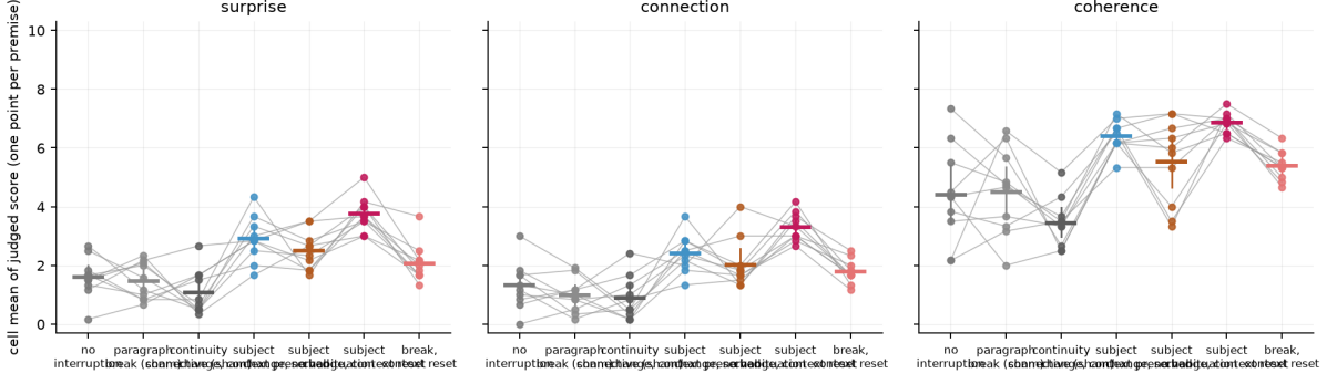
Figure 8: What carries the effect at period 300: no interruption, a paragraph break (sham), a continuity connective (sham), the subject change on the preserved context, the subject change without habituation, the subject change on a reset context, and a break on a reset context; one point per premise.
