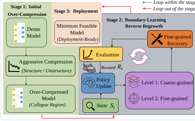
Figure 3: BEIDGE: Boundary-Learning Reverse Regrowth Framework. The framework first over-compresses the model to expose the compression boundary, then performs a hierarchical reverse regrowth process to restore critical structures, and identifies the minimum feasible model for deployment.
