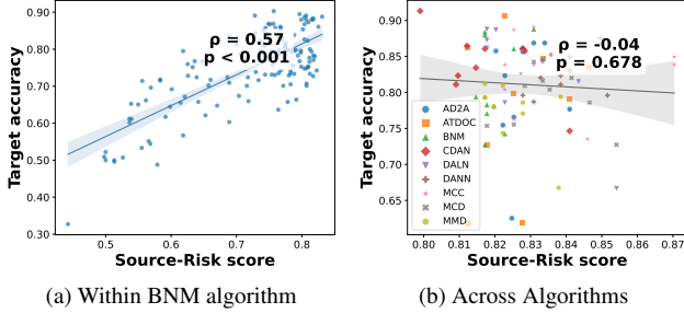
Figure 6. Spearman correlation ( \rho ) between Source-Risk scores and target accuracy on ADNI-1 → ADNI-2. Each point is a check-point. (a) Within BNM algorithm, the correlation is moderate. (b) Across all algorithms, it collapses to near zero.
