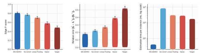
Fig. 5. Ablation study isolating the contribution of barycentric fusion and algorithm unrolling, measured by F -score, relative error, and per-instance estimation time.
