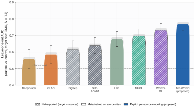
Fig. 12. Leave-one-out AUC for autism-versus-control classification using graph-spectral features of the learned target-site connectivity graph.
