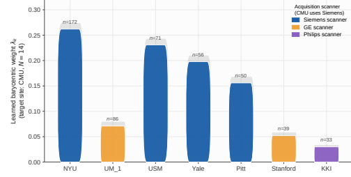
Fig. 14. Barycentric weights learned by MS-WDRO across the seven ABIDE I source sites when estimating the CMU target graph, annotated by acquisition scanner vendor.
