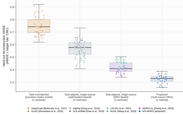
Fig. 16. Reconstruction NMSE aggregated by methodological family.
