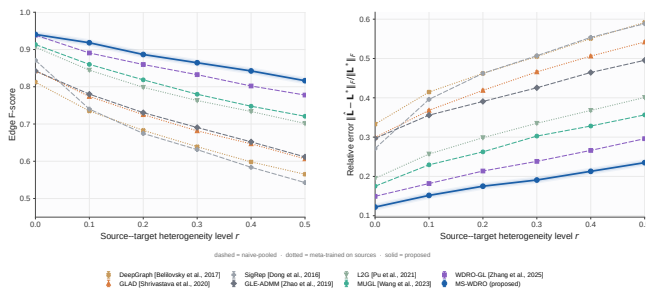
Fig. 3. Edge F -score and relative Frobenius error versus source-target heterogeneity (rewiring rate) r ( N = 20 , M = 5 , n_{\text{tgt}} = 20 ).
