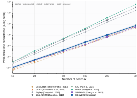
Fig. 9. Wall-clock time per instance versus number of nodes N (log-log scale).
