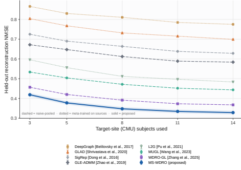
Fig. 11. Held-out reconstruction NMSE versus number of target-site (CMU) subjects used for estimation.
