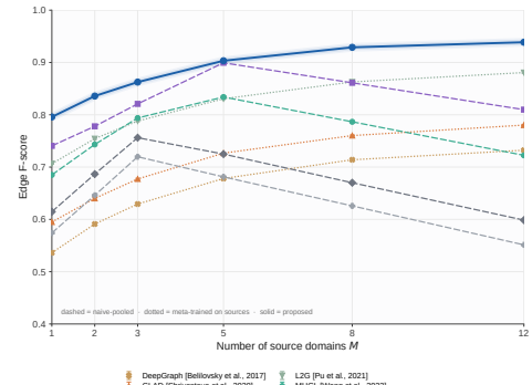
Fig. 4. Edge F -score versus number of source domains M ( N = 20 , r = 0.3 , n_{\text{tgt}} = 20 ). Naive-pooling baselines exhibit negative transfer beyond M \approx 5 .
