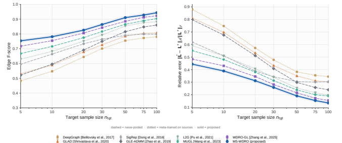
Fig. 2. Edge F -score and relative Frobenius error versus target sample size n_{\text{tgt}} , averaged over 50 trials ( N = 20 , M = 5 , r = 0.3 ). Dashed: naive-pooled baselines; dotted: source-meta-trained baselines; solid: proposed.
