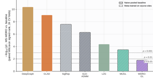
Fig. 13. Statistical significance ( -\log_{10} p , paired Wilcoxon signed-rank test, 24 cross-validation folds) of MS-WDRO’s improvement over each baseline.
