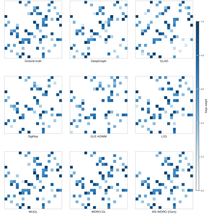
Fig. 8. Recovered adjacency matrices for all eight methods on a representative trial, alongside the ground-truth graph.
