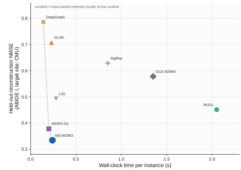
Fig. 15. Held-out reconstruction NMSE versus per-instance wall-clock time on ABIDE I; MS-WDRO and WDRO-GL jointly define the Pareto frontier.
