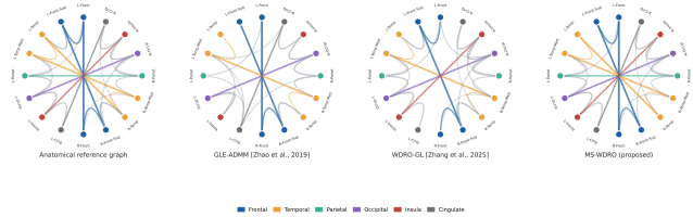
Fig. 17. Circular connectograms of the recovered CMU functional network for a representative classical baseline (GLE-ADMM), the strongest single-source baseline (WDRO-GL), and MS-WDRO, alongside a structural-proximity reference graph.
