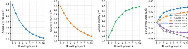
Fig. 6. Layer-wise evolution of the four learned parameters over K_\ell = 10 unrolled layers: ambiguity radius \epsilon^{(k)} (objective-level; decreasing), sparsity regularization coefficient \rho^{(k)} (objective-level; decreasing), ADMM penalty \varrho^{(k)} (algorithm-level; increasing), and barycentric weights \lambda_m^{(k)} , m = 1, \dots, M , for M = 5 sources.
