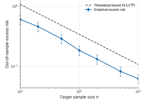
Fig. 7. Empirical out-of-sample excess risk versus target sample size n , compared against the theoretical \mathcal{O}(1/\sqrt{n}) bound of Theorem 3.3 (log-log scale).
