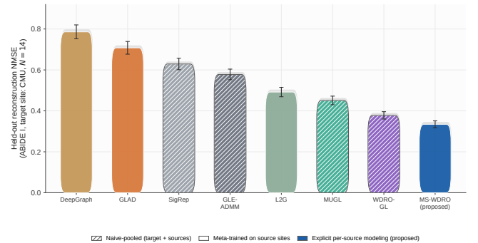
Fig. 10. Held-out reconstruction NMSE on ABIDE I (target site: CMU, N = 14 ) for all eight methods. Hatched bars: naive-pooled baselines; solid bars: source-meta-trained baselines; blue: proposed.
