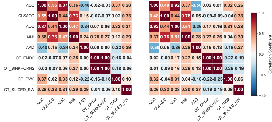
Fig. 4: Pairwise correlation between 9 evaluation metrics for the percentage of features selected in the range (0.5%–5%). The left plot reports Pearson correlations; and the right plot reports Spearman. Red cells mark metric-pair that ranks the feature selection methods consistently in the same direction, blue cells represent a pair that ranks them in opposite directions.
