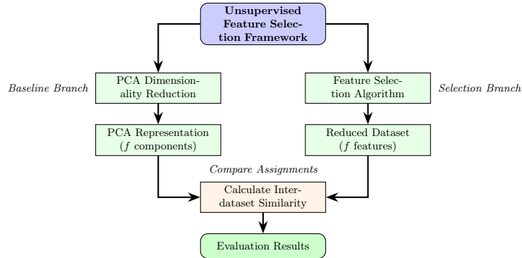
Fig. 1: Proposed method for truly unsupervised evaluation of feature selection.
