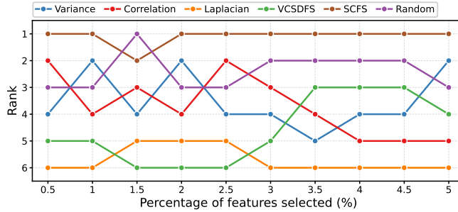
Fig. 3: Ranking produced by Ot_Sliced_SW for Isolet dataset as a function of the percentage of features selected. 1 represents highest rank and 6 represents lowest rank.
