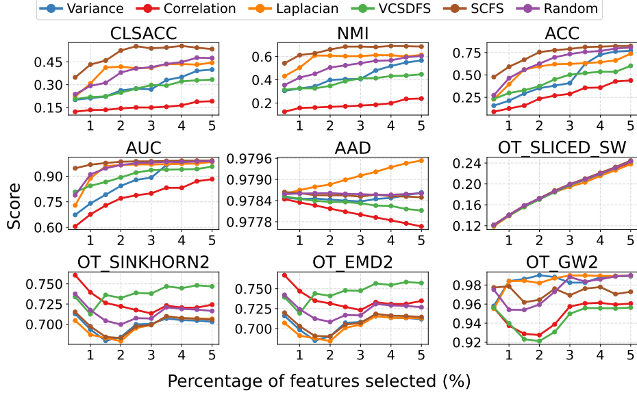
Fig. 2: Performance curves of the nine evaluation metrics on Isolet as a function of the percentage of features selected. For all measures, higher is better (distances are converted to similarities for OT-measures).
