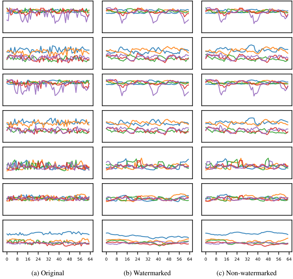
Figure 6: Visualization of original and generated samples on the ETTh dataset with length 64.
