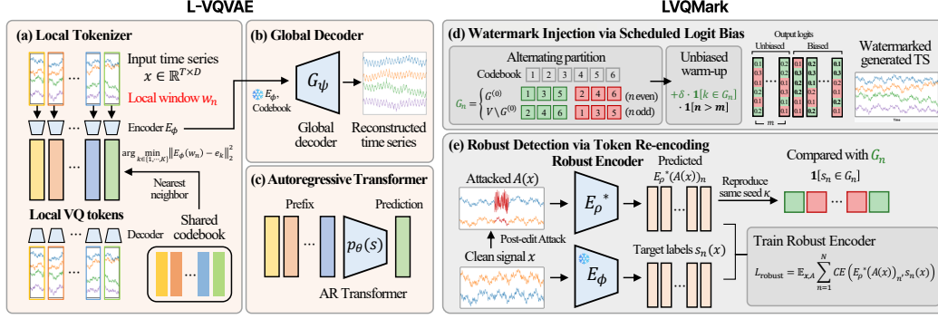
Figure 2: Overview of L-VQVAE and LVQMark. (a) The local tokenizer encodes each temporal window into a discrete VQ token. (b) The global decoder reconstructs the time series from the token sequence. (c) An autoregressive transformer models the token distribution. (d) Watermark injection via scheduled logit bias with alternating partition and unbiased warm-up. (e) Robust detection via token re-encoding, where E_\rho^* recovers clean token assignments from the attacked signal for the green-ratio test.
