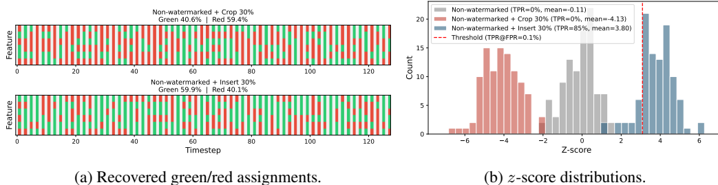
Figure 1: Bidirectional drift of the null on non-watermarked samples (TimeWak [17], Stocks). Crop and insert push the recovered tokens (a) and the resulting z -score (b) in opposite directions, with insert crossing the clean-calibrated threshold and yielding an 85% false-positive rate.
