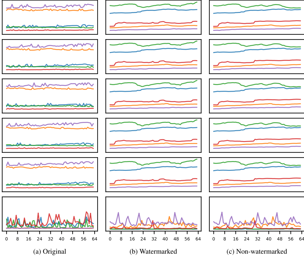
Figure 5: Visualization of original and generated samples on the Stocks dataset with length 64.
