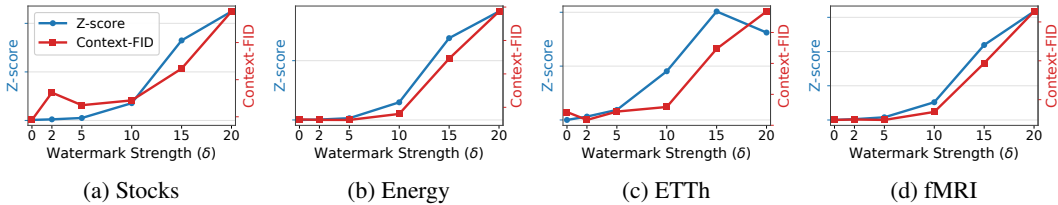
Figure 4: Z-score and Context-FID across watermark strength \delta for 64-length
