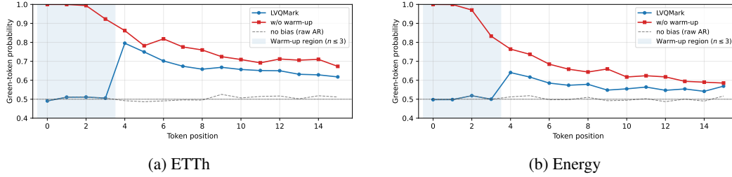
Figure 3: Per-position green-token probability ( T=64 , \delta=10 ). Shaded region: warm-up positions ( n \leq 3 ) where the logit bias is suppressed.
