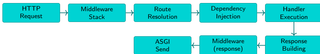
Figure 2 Request processing pipeline. The request flows left to right through the middleware stack, route resolution, dependency injection, and handler execution. The response flows back through the middleware stack before being sent to the client.
