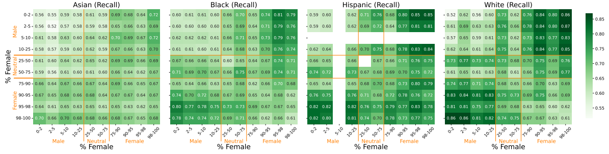
Figure 2: Recall of predicting romantic relationships from Llama2-7B for subset of the dataset where characters originally have different genders. Horizontal and vertical axes denote % female of the name replacing an originally female and male character name from the dialogue. The upper-triangle (lower-triangle) shows the scores when names are replaced preserving (swapping) the genders of characters’ names as-is in the original conversation. We consider the names with lesser % female as male names for determining gender preservation for name-replacement.
