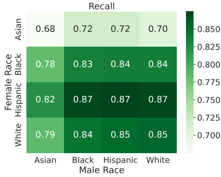
Figure 3: Recall of predicting romantic relationships from Llama2-7B for subset of the dataset where characters have different genders and are replaced with names associated with different races/ethnicities.
