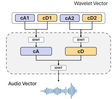
(c) Block of Multi-Level Inverse Discrete Wavelet Transform
