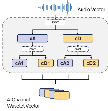
(a) Block of Multi-Level Discrete Wavelet Transform
