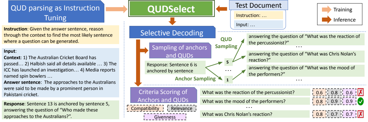
Figure 2: Overview of our QUDSELECT framework.
