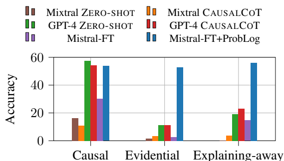
Figure 1: Percentage of instances solved correctly for each Bayesian reasoning type . The neuro-symbolic Mistral-FT+ProbLog approach is robust against the inherent difficulties of different reasoning types.
