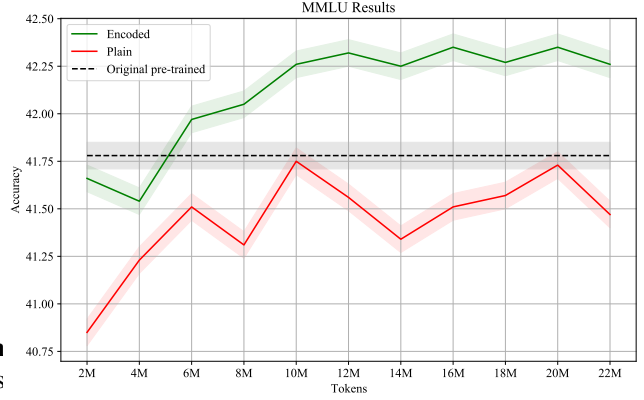
Figure 2: MMLU Accuracy of Llama2-7B. Continuing self-supervised pretraining on web-curated text tokens, when numbers are encoded with NúmeroLogic, helps improve the performance beyond the pretrained model or a model trained on the same text with plain numbers.
