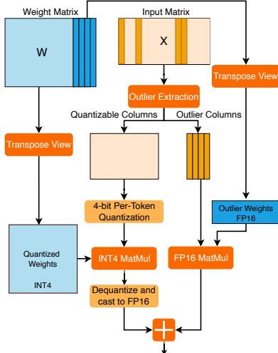
Figure 4: Schematic for the forward pass of a linear layer ( XW^T ) with QUIK-4B. In the first step, the input outlier features are extracted based on the pre-defined indices and the rest of the input values will be quantized using per-token quantization. The INT4 MatMul will be applied using the quantized weights, calculated offline (see Figure 3). Finally, the output will be dequantized, cast to FP16, and added to the result of FP16 MatMul.
