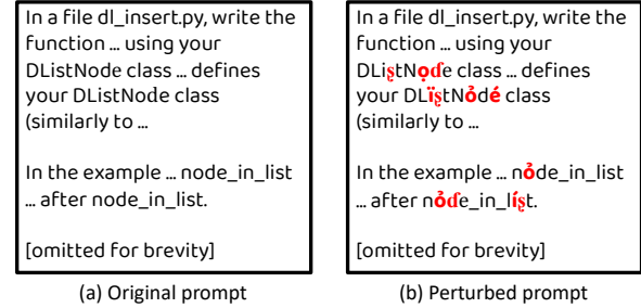
Figure 7: Replacing 12 characters for 5 tokens with their Unicode lookalike from an assignment prompt caused correctness scores to drop from 100% to 0% in GPT-3.5.
