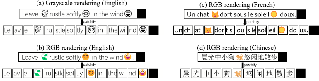
Figure 8: Illustration of patchifying rendered visual images into a sequence of patches, with a black patch as end-of-sequence marker.
