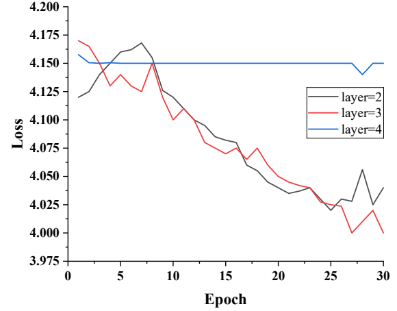
Figure 4: The loss trends during pre-training with different graph encoding layers settings.
