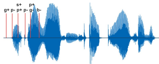
Figure 1: Example of Acoustic Landmark (2-gram concat landmark (g+p-), (s+p+), (p+p-), ..., (g-b-)), Landmarks are extracted from abrupt changes in the speech signal. They can discretize speech into a series of tokens that possess linguistic significance.
