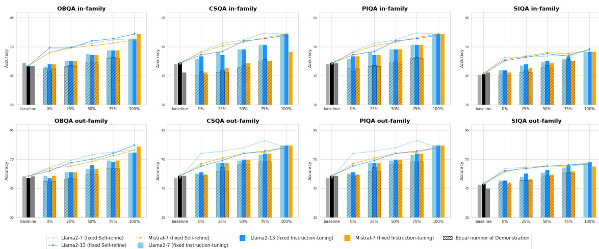
Figure 4: Accuracies (%) on the test set of benchmarks. The Self-refine Instruction-tuning performed on different splits (see Appendix C.1 for major details).
