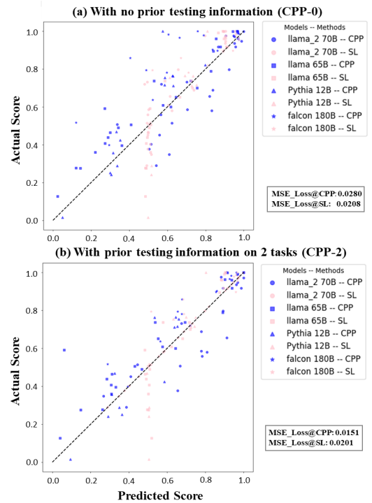
Figure 5: Comparison of the predictive performance of collaborative performance prediction (CPP) versus traditional scaling laws (SL) for LLMs: (a) CPP-0, with no prior testing information, and (b) CPP-2, with prior testing on two tasks.
