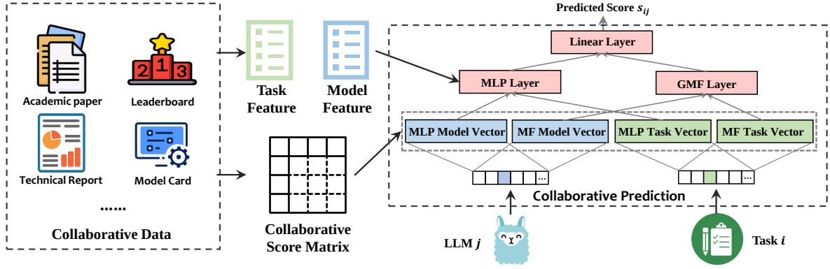
Figure 1: Framework for Collaborative Performance Prediction of Large Language Models. This schematic delineates two principal components: (1) Collaborative Data, which encompasses a score matrix illustrating the performance of various LLMs across downstream tasks, along with external descriptive factors of both models and tasks; (2) Collaborative Prediction Method, given the model and task IDs to leverage this collaborative data, enabling accurate score prediction.
