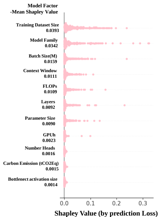
Figure 11: Instance Distribution of the model factor Shapley value. X-axis represents the Shapley value, which indicates the degree of prediction loss change; Y-axis indicates the factor names in order of importance from top to bottom. Each point represents an instance.
