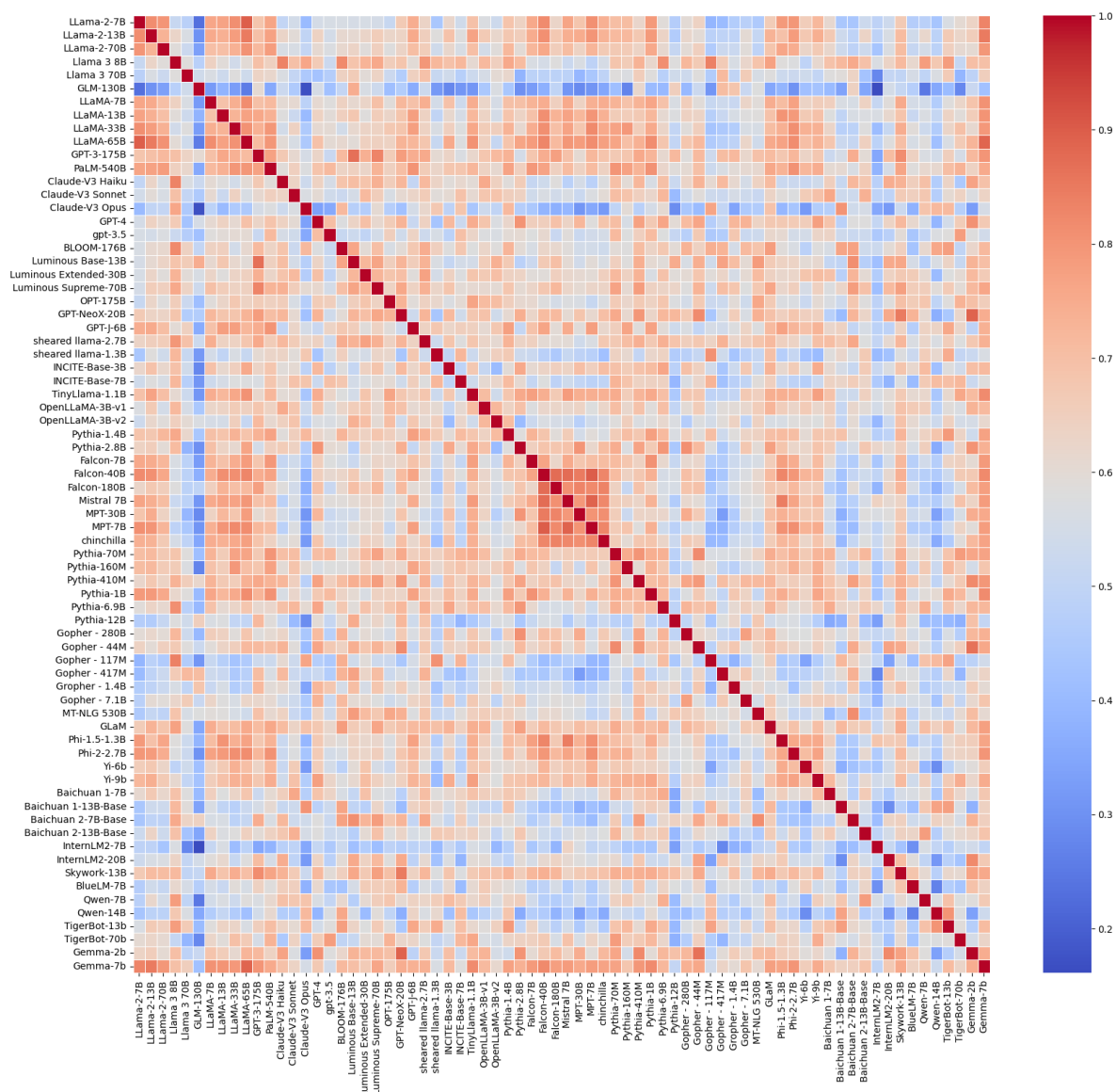
Figure 13: The correlation heatmap of impacts of different models on prediction performance.
