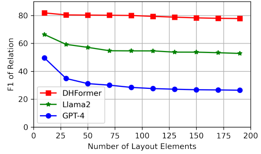
Figure 5: Comparison of the DHFormer and LLMs, in terms of model performance in relation to variations in document length.
