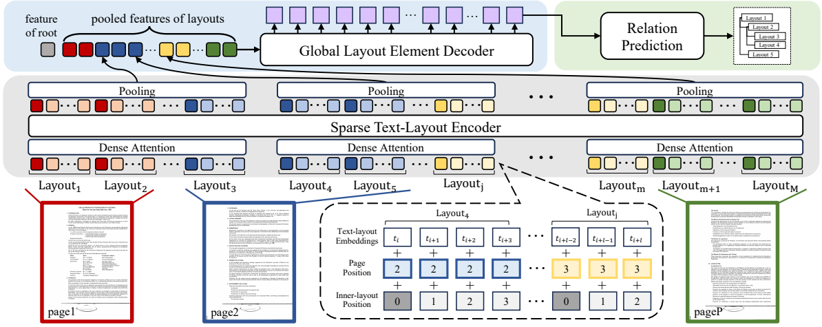
Figure 4: An overview of DHFormer. The sparse text-layout encoder efficiently enriches the input representations with fine-grained contexts. Then the decoder takes as input the pooled layout features of the document and reasons at global range. Finally the relations are predicted based on features of layout elements.
