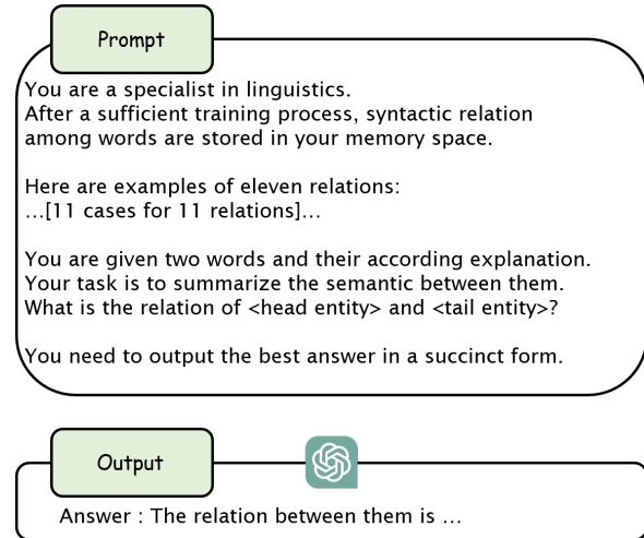
Figure 6: Prompt in the open-domain knowledge alignment setting for WN18RR.
